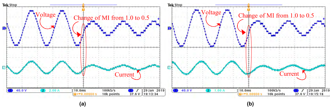
FIGURE 11. Output voltage and current waveform with change of modulation index from 1.0 to 0.5 with (a) R = 100\ \Omega [Scales: v_o = 40\text{V/div} , i_o = 2\text{A/div} ], and (b) R=100\ \Omega, L=100\text{mH} , [Scales: v_o = 40\text{V/div} , i_o = 1\text{A/div} ].
