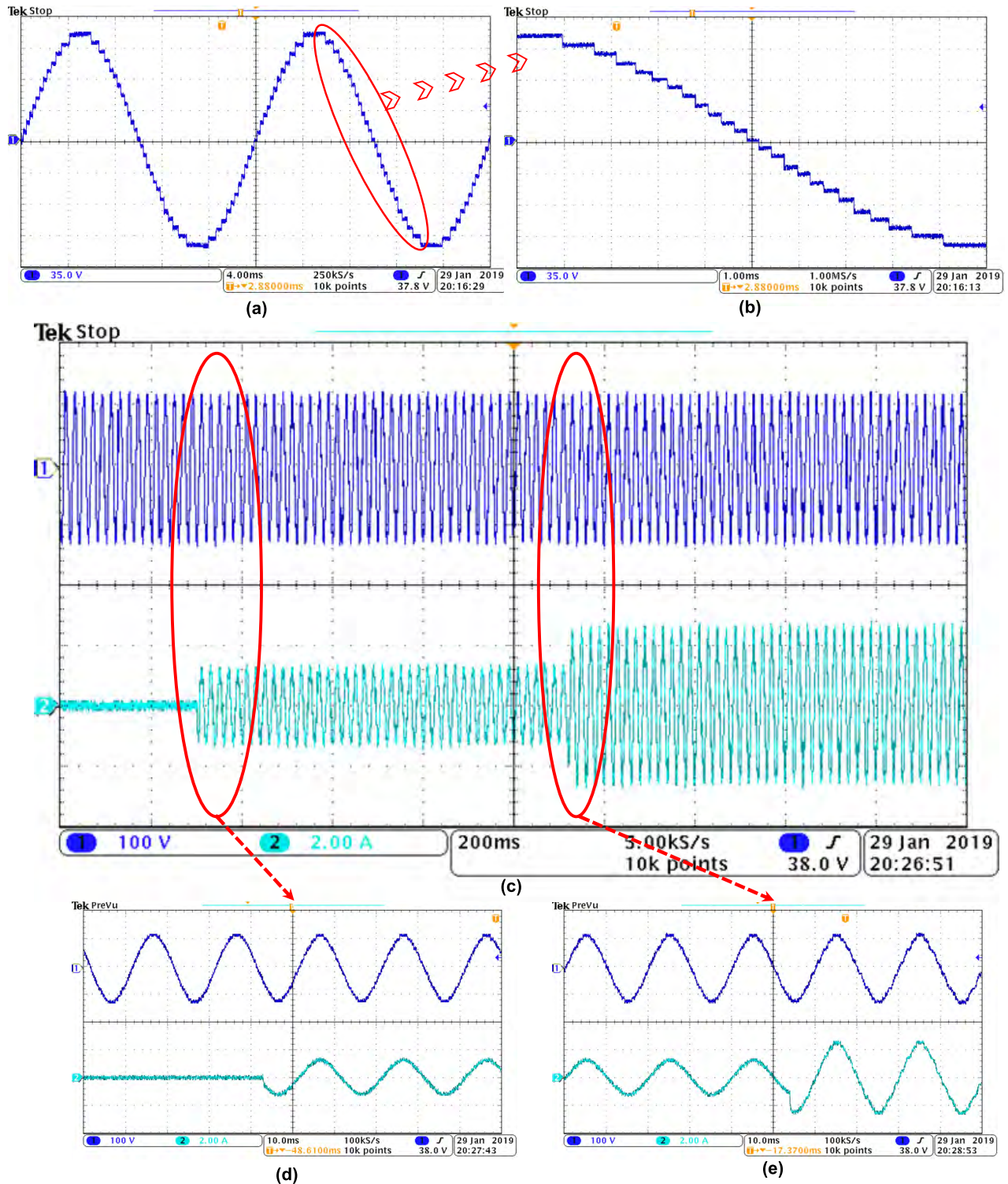
FIGURE 12. Experimental results for (a) 25 level output voltage waveform, (b) zoomed view of output voltage, (c) output voltage and current waveform with different resistive load [scale: v_o = 100\text{V/div} , i_o = 2\text{A/div} ], (d) transient-state waveforms with change of load from R=0 to R=100\ \Omega , [scale: v_o = 100\text{V/div} , i_o = 2\text{A/div} ], (e) transient-state waveforms with change of load from R=100\ \Omega to R=50\ \Omega , [scale: v_o = 40\text{V/div} , i_o = 2\text{A/div} ].
